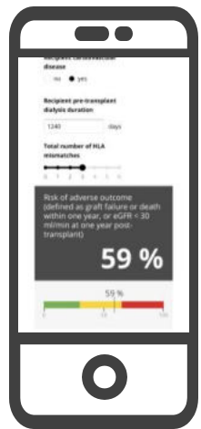
pre-image.eu/calculator AUC = 0.63
