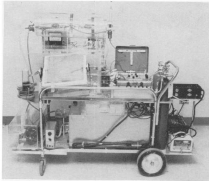
FIG. 3. Photograph of transportable renal preservation unit.
